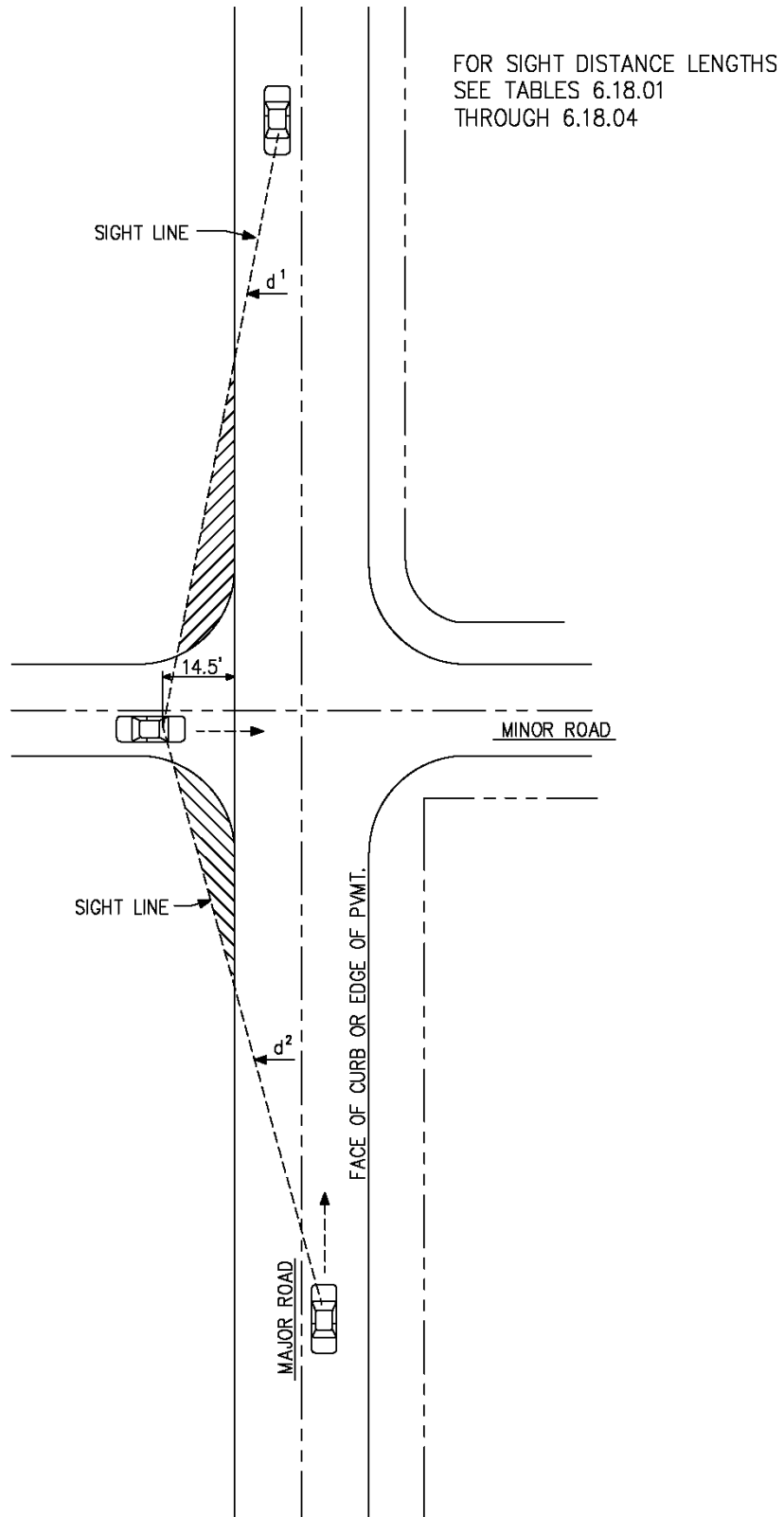
FIGURE 6.18.02 Intersection Sight Lines Case 2
